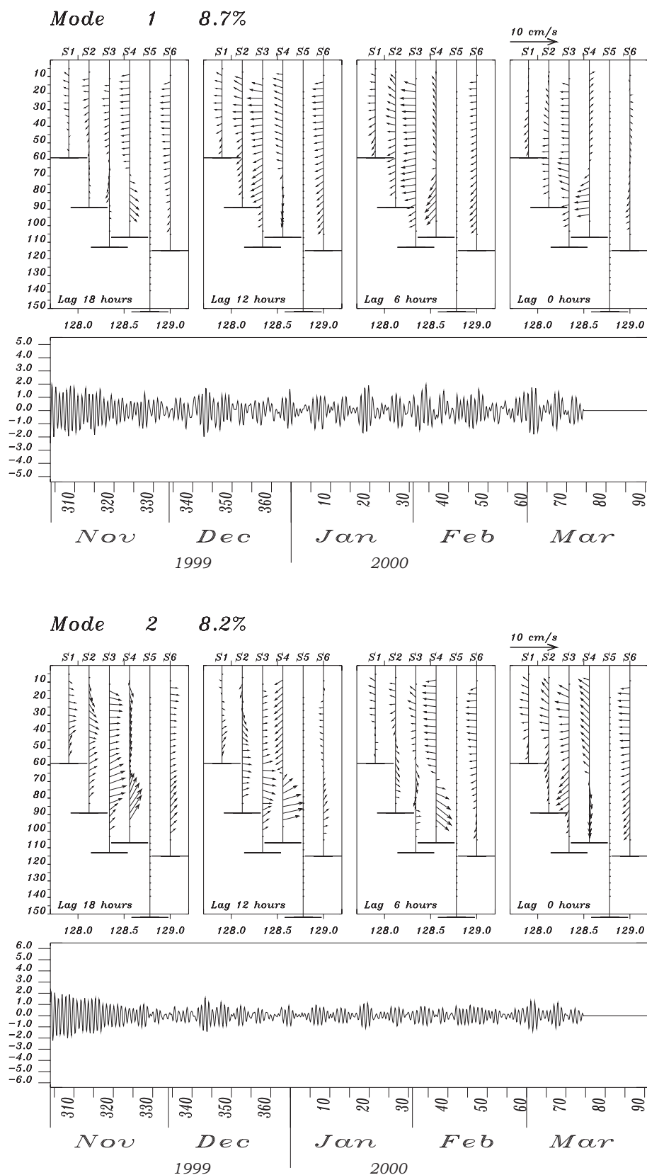
Figure 4. The same as Figure 3, except using data only during winter. The winter extended EOF does not contain the clockwise rotation as the summer data. Thus most of the variability at the 1.10 cpd is not associated with inertial oscillations in winter.
