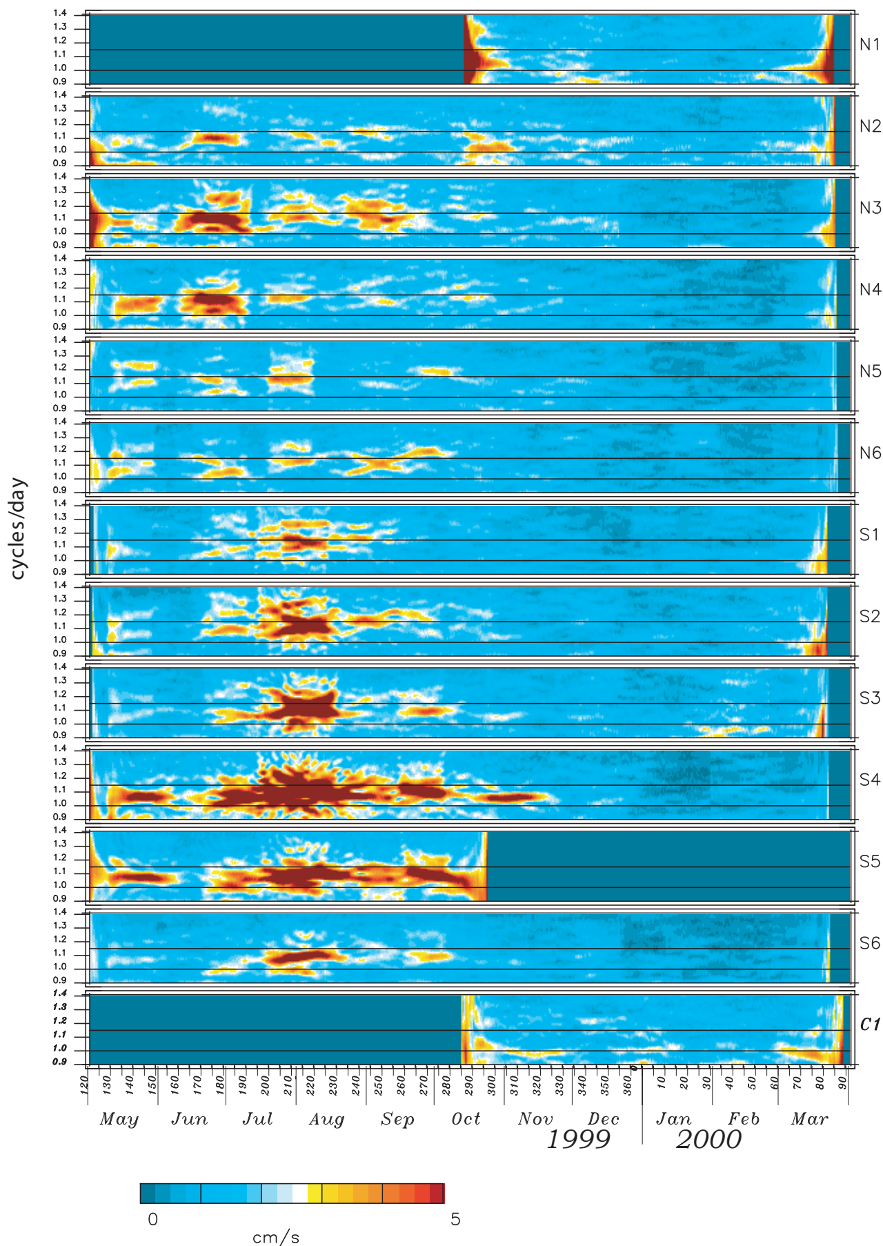
Plate 2. The time-varying amplitude spectra using a 20 day window indicates the frequency at which the energy is occurring. The 20 day window provides a frequency resolution of 0.05 cpd. The two horizontal lines in each plot are at the 1 cpd and 1.15 cpd frequencies. Most of the energy is at a frequency slightly less than the local inertial frequency.
