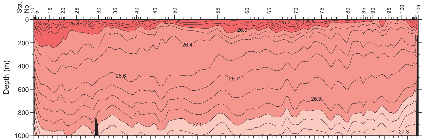
\sigma_0 (red), \sigma_2 (green), \sigma_4 (blue) (kg/m 3 ) for I5P 33°S
