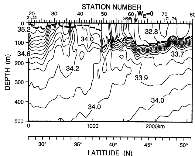
Figure 15. Salinity along 152°W in May 1984. The heavy dashed line shows the mixed layer depth defined by the maximum Väisälä frequency in vertical. The arrow shows where the monthly mean vertical Ekman velocity equals zero in May 1984. The southern boundary of the subarctic frontal zone occurs near station 52.
