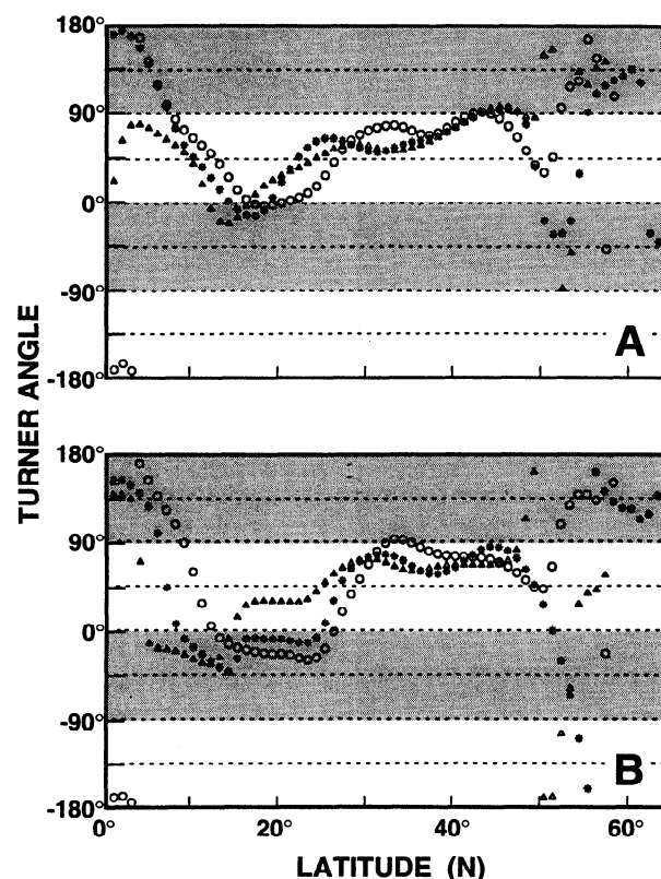
Figure 7. Turner angle at 10-m depth from Levitus's [1982] (a) winter and (b) summer data. Triangles, asterisks, and circles are the Turner angles in the western (165°E), central (175°W), and eastern (140°E) North Pacific, respectively. Shaded areas show where salinity gradients dominate. Temperature gradients dominate in unshaded areas.
