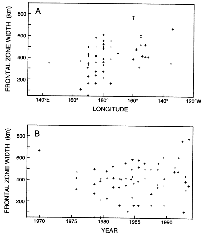
Figure 11. (a) Spatial and (b) temporal variations of frontal zone width in kilometers from 63 sections which completely cross the subarctic frontal zone.
