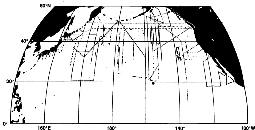
Figure 8. Map of conductivity-temperature-depth/salinity-temperature-depth (CTD/STD) stations used in section 3. In total, there are 3880 stations and 72 cross-front sections from 36 research cruises occupied between 1968 and 1993.
