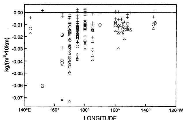
Figure 16. Mean \alpha\Delta_y T (triangles), \beta\Delta_y S (circles), and \Delta_y\sigma_\theta (crosses) at 10-m depth in the subarctic frontal zone from 63 complete cross-front CTD/STD sections. Units are kilograms per cubic meter per 10 km.
