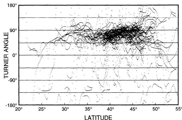
Figure 17. Turner angles along 72 CTD/STD sections. Temperature and salinity are horizontally smoothed with a Gaussian filter of 2° latitude width before calculating the Turner angles. Most of the angles are between 45° and 90° in the latitude range of 25° to 45°N, which agrees with Levitus 's [1982] data in section 2.4, although the synoptic data are much noisier.
