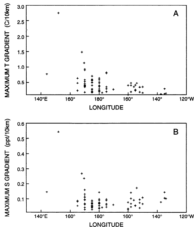
Figure 12. (a) Maximum temperature and (b) maximum salinity gradients at 10-m depth in the subarctic frontal zone as functions of longitude. Units are degrees Celsius per 10 km and parts per thousand per 10 km for temperature and salinity, respectively.
