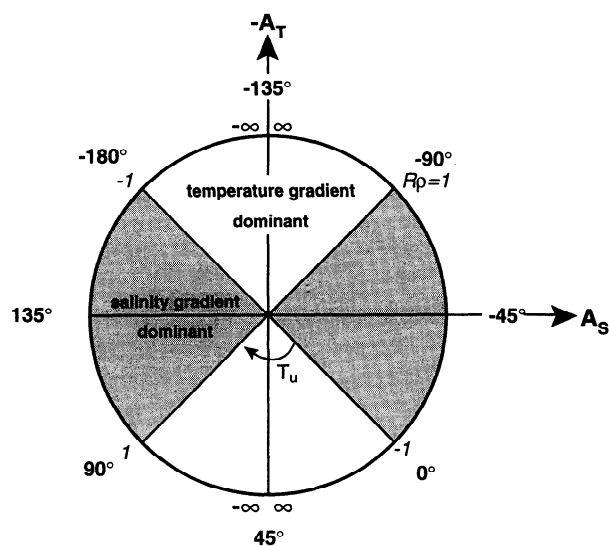
Figure 6. The plane -A_T = -\alpha \partial_y T versus A_S = \beta \partial_y S . Lines of constant R_p radiate outward at a constant angle from the origin. Some values are shown outside the circle. Increasing Turner angles are in the direction of the arrow. The areas where the salinity gradient contribution to density gradient exceeds temperature's contribution are shaded. Temperature gradients dominate in unshaded areas.
