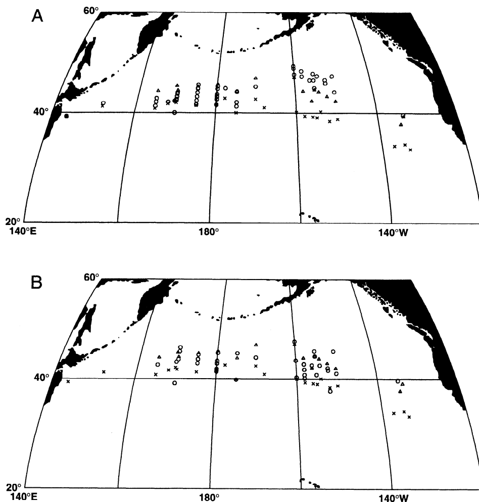
Figure 18. (a) The northern boundary of the North Pacific Intermediate Water (circles) relative to the northern (triangles) and southern (crosses) boundaries of the subarctic frontal zone. (b) The northern onset of the shallow salinity minimum (circles) relative to the southern (crosses) and northern (triangles) boundaries of the subarctic frontal zone.
