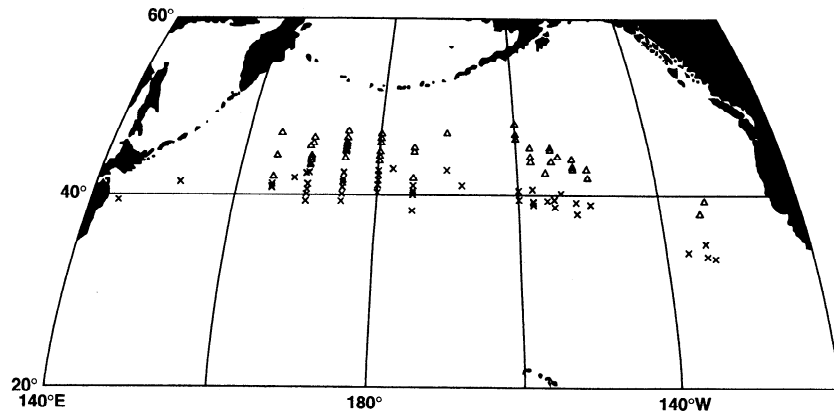
Figure 10. The southern (crosses) and northern (triangles) boundaries of the subarctic frontal zone defined by the outcropping of the subarctic halocline (see text) for 72 cross-front CTD/STD sections in the North Pacific.
