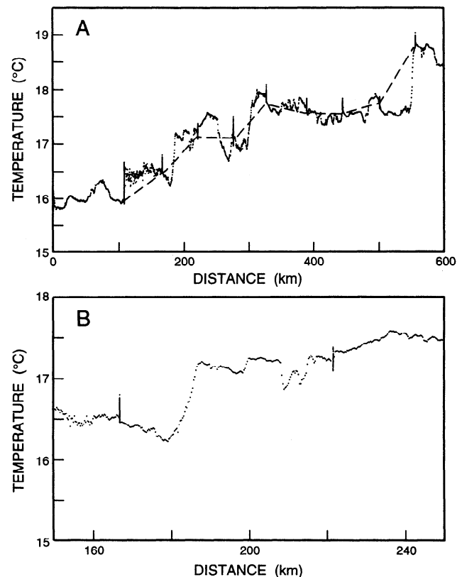
Figure 14. (a) Underway temperature from 34.6°N to 30.0°N along 135°W in June 1991. Heavy dashed line is a contour of the sea surface temperature from the temperature at CTD stations. (b) A single front at 33.75°N (near distance 180 km) within the subarctic frontal zone defined by salinity structure from CTD station data.
