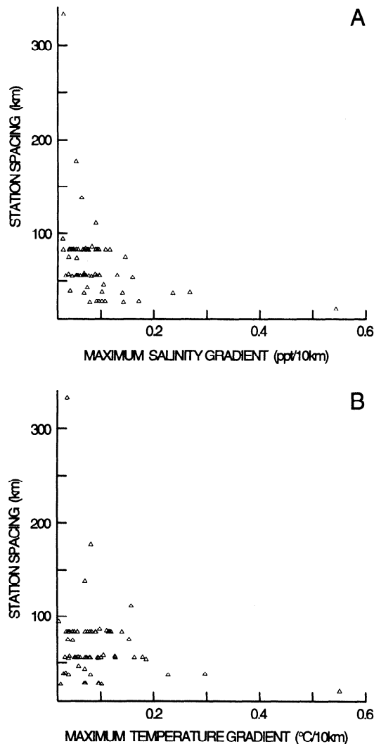
Figure 13. (a) Maximum salinity and (b) maximum temperature gradients in the subarctic frontal zone as functions of the station spacing near the frontal zone for each of the CTD/STD surveys. The mean station spacing over the 72 sections is 66 km.
