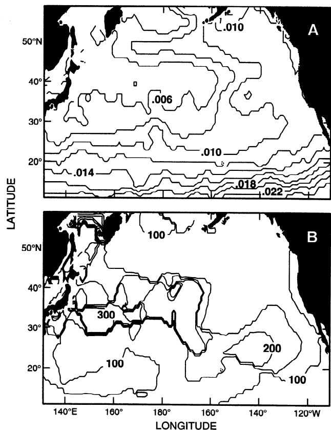
Figure 5. (a) Magnitude of the largest vertical maximum of the Väisälä frequency in the upper 400 m in winter from Levitus's [1982] data. Units are radians per second. (b) Depth (in meters) of the largest vertical maximum, with a contour interval of 100 m.
