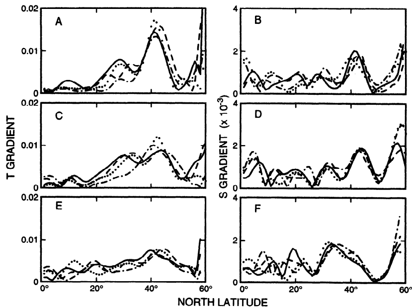
Figure 3. Horizontal temperature and salinity gradients (a–b) along 165°E, (c–d) along 170°W, and (e–f) along 140°E from Levitus's [1982] winter (solid lines), spring (dotted lines), summer (dashed-dotted lines), and fall (dashed lines) data at a depth of 10 m. Units are degrees Celsius per kilometer and parts per thousand per kilometer for temperature and salinity, respectively.
