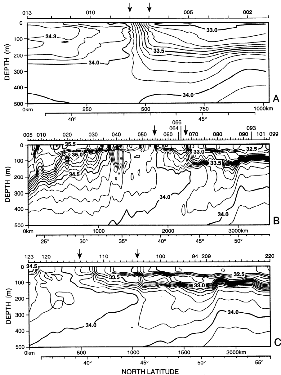
Figure 9. Salinity (a) along 170°E in July 1985, (b) along 158°W in September 1991, and (c) along 155°W in September 1991, as examples for the definition of the northern and southern boundaries of the subarctic frontal zone. See text for the definition. The southern and northern boundaries are indicated by arrows. The three sections show the different frontal structures.
