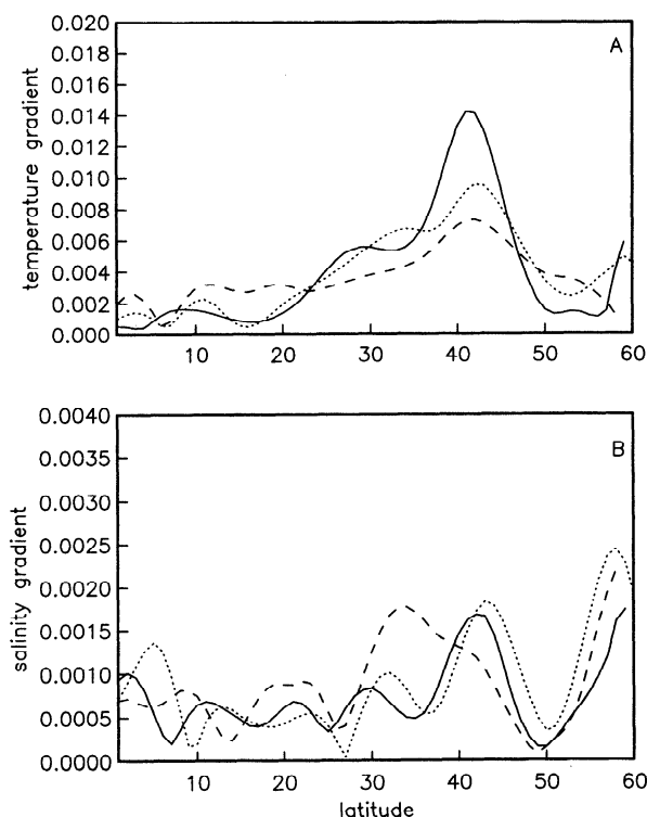
Figure 1. Horizontal gradients of Levitus's [1982] annual mean (a) temperature and (b) salinity at 10-m depth along meridians of 165°E (solid lines), 170°W (dotted lines), and 140°W (dashed lines), which represent the western, central, and eastern North Pacific, respectively. Units of temperature gradients are degrees Celsius per kilometer. Units of salinity gradient are parts per thousand per kilometer.
