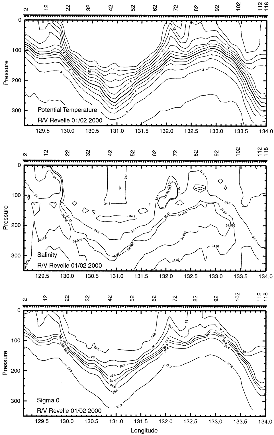
FIG. 5c. Jan 2000 Revelle section of potential temperature, salinity, and sigma- \theta along 37°45'N.
