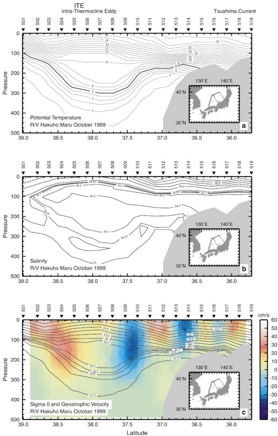
FIG. 3. Hakuho-Maru section, obtained in Oct 1999, showing the ITE; potential temperature (a), salinity (b), and sigma- \theta density (c). Superimposed on the sigma- \theta section is the geostrophic current normal to the section relative to 1000 db or to the seafloor where shallower than 1000 db.
