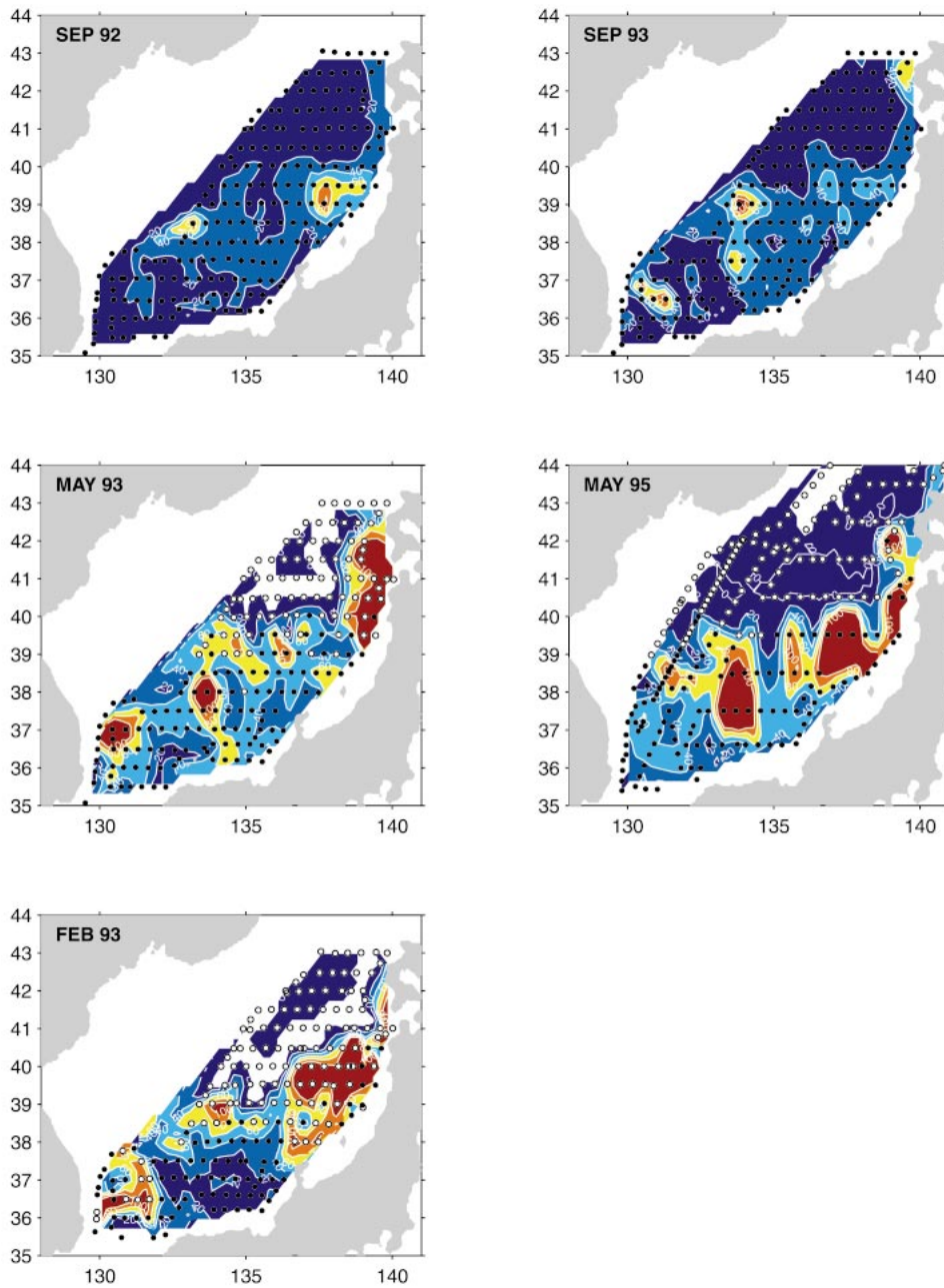
FIG. 9. Distance (in m) between the 8° and 11°C isotherms as seen in five comprehensive surveys by AXBT Sep 1992, 1993; May 1993, 1995; and Feb 1993. Open circles are profiles where the sea surface temperature is colder than 11°C.
