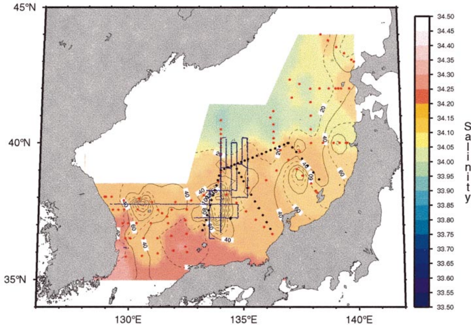
FIG. 6. Map of the layer thickness (m) between the 8° and 11°C isotherms as observed during the Revelle cruises of May–Jul 1999 and Jan–Feb 2000, and from the Hakuho-Marui in Oct 1999. The color coding shows mean salinity within this temperature interval. Jul Revelle stations are shown as red dots; Hakuho-Marui are shown as black dots; the SeaSoar lines of the May and Jan Revelle cruises are shown as dotted lines.
