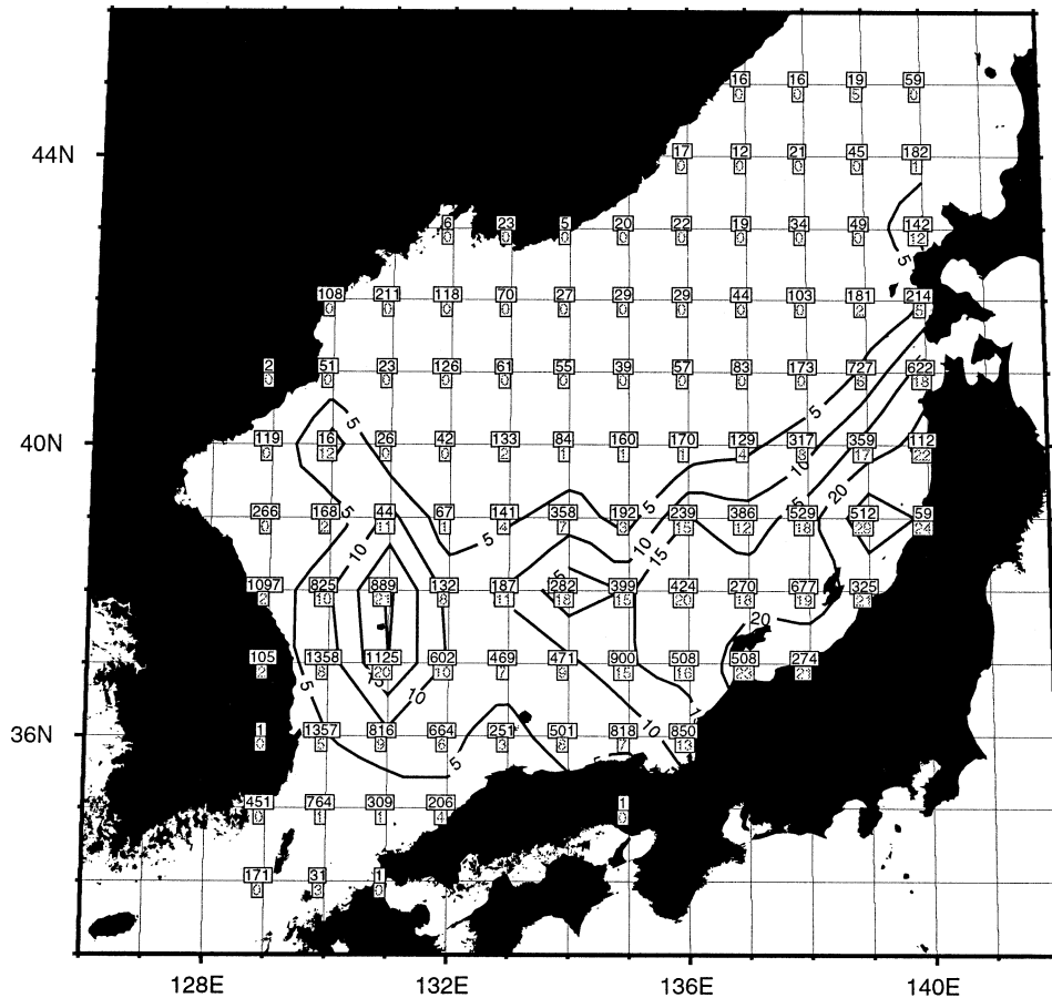
FIG. 8. Percentage of occurrence of profiles displaying ITE characteristics as denoted by more than 80 m separation between the 8° and 11°C isotherms. The total number of stations inspected was 29 653, drawn from the 1926–94 NODC dataset, the 1995–97 (Japan Meteorological Agency) archive, and the 1999 Revelle and Hakuho-Maru data. The data is binned in 1° lat by 1° lon boxes. For each box the upper value is the total number of stations inspected, and the number below that value is the percentage displaying ITE characteristics. The values are positioned in the center of their lat/lon box.
