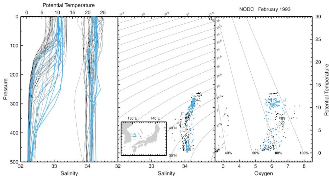
FIG. 10. The potential temperature and salinity profiles (a) and potential temperature vs salinity (b) and oxygen (c) obtained at stations off the Korean coast, Feb 1993 (NODC dataset). Stations displaying thick surface layers with characteristics similar to those of the ITE are shown as thicker lines or larger dots.
