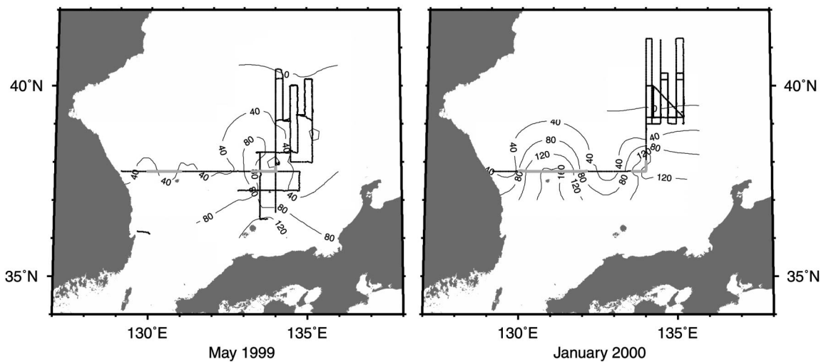
FIG. 5a. Map of SeaSoar sections in May 1999 and Jan 2000 obtained by the RV Revelle . The contours are of the 12°C isotherm depth.
