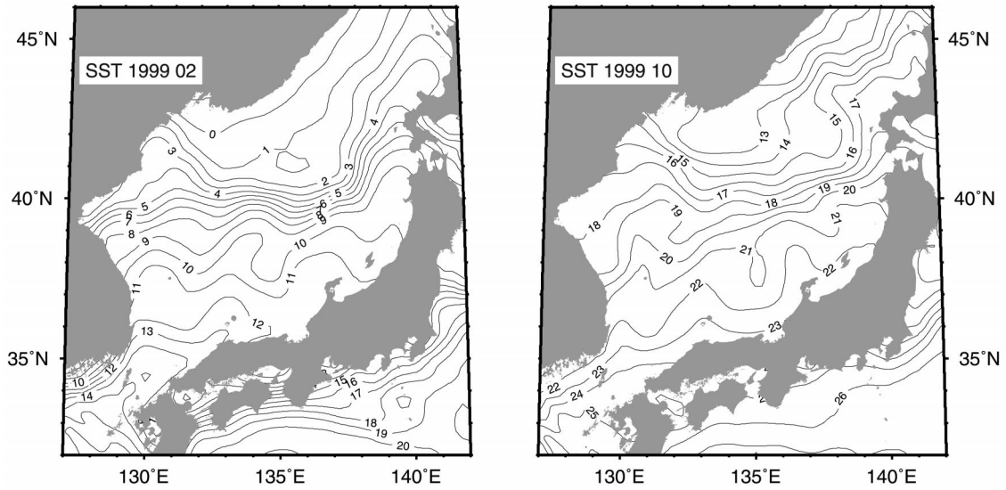
FIG. 2. Feb 1999 and Oct 1999 sea surface temperature maps. The data shown are for a monthly average of the daily sea surface temperature data analysis from the Japan Meteorological Agency. The analysis has a resolution of a quarter degree and combines sea surface observations by NOAA with in situ observations by ships and buoys. The data was obtained from the NEAR-GOOS Regional Delayed Mode Data Base operated by the Japan Oceanographic Data Center.
