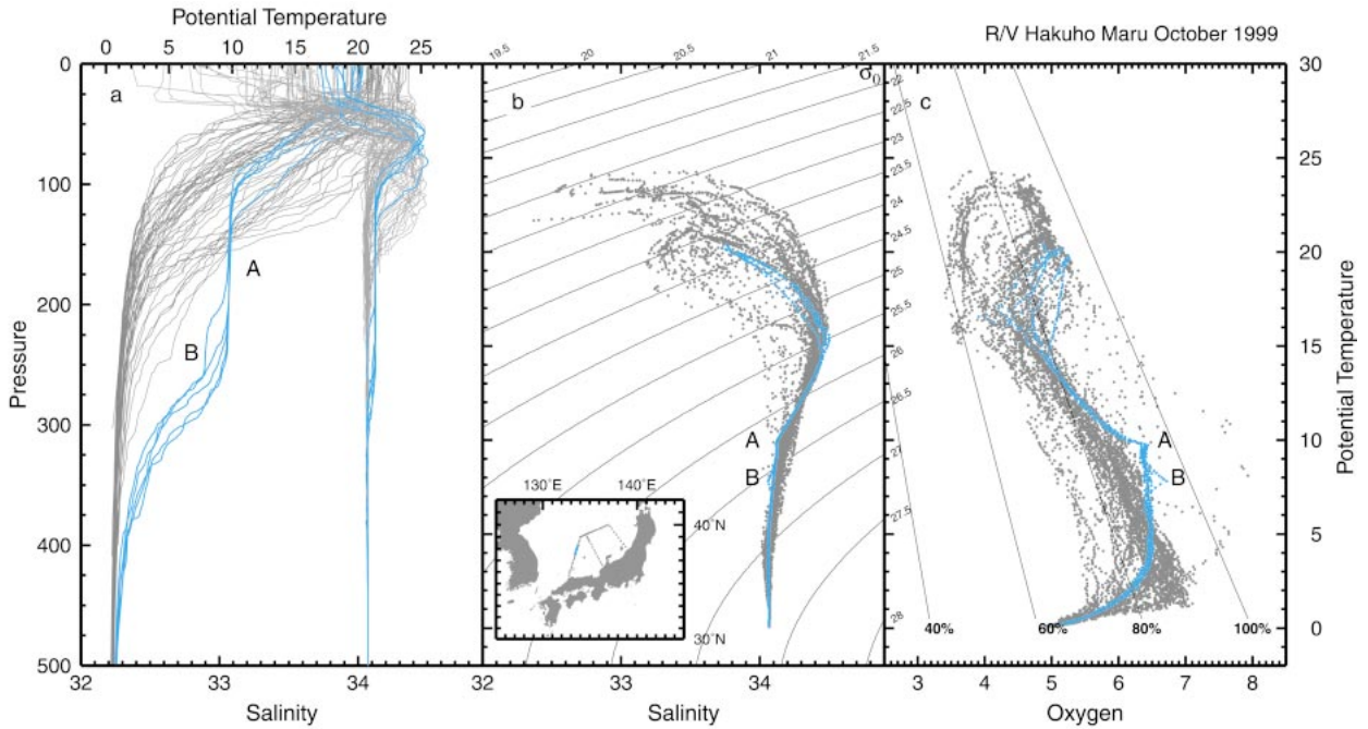
FIG. 4. The potential temperature and salinity profiles (a), potential temperature vs salinity (b), and potential temperature vs oxygen (c). The stations 505–509 defining the ITEs are shown in blue.
