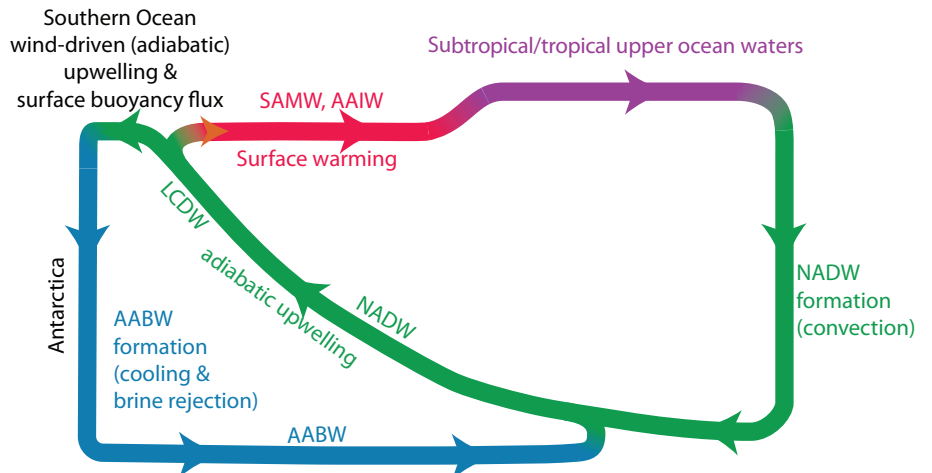
(c) Southern Ocean upwelling (missing low latitude upwelling)
