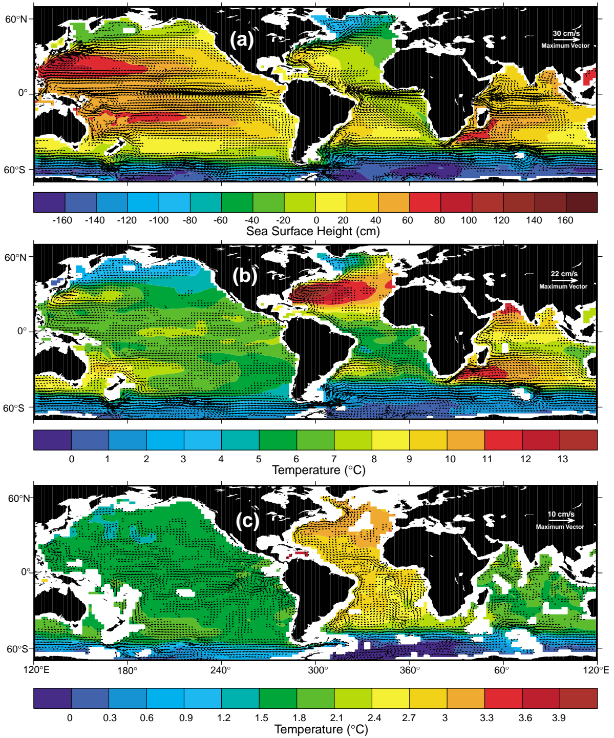
Plate 7.1.9 (a) Mean surface velocity field superimposed on the mean sea surface height field (in cm) of the constrained MIT model. In (b) and (c) the mean flow field at 610 and 2450 m depth are superimposed on the estimated mean temperature field at those levels.
