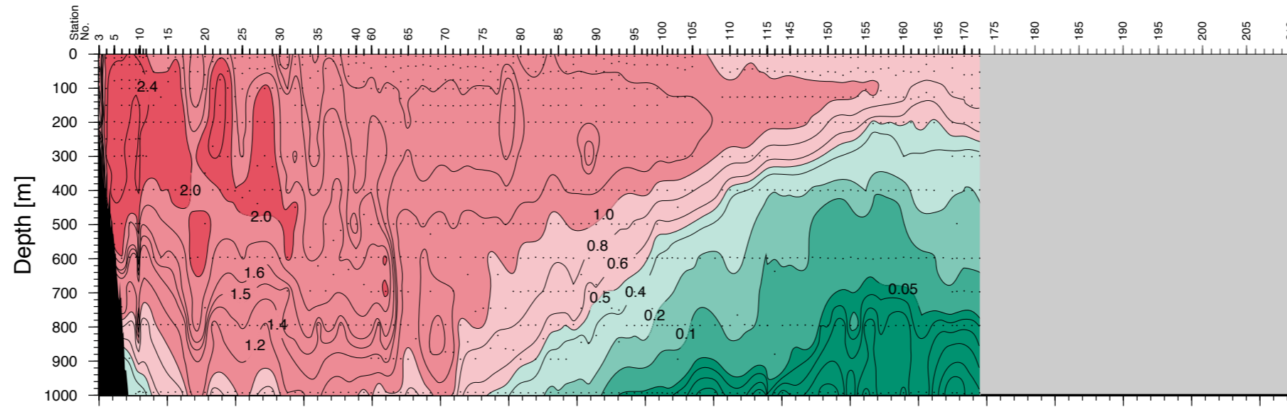
CFC-11 [pM/kg] for A17
