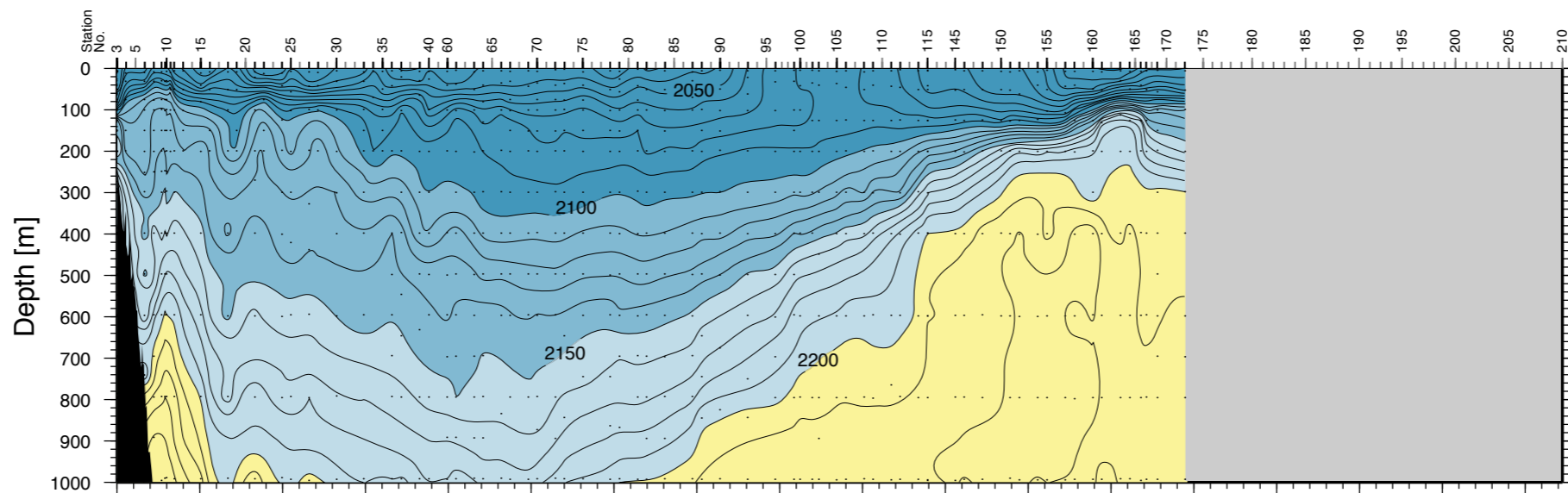
Total CO 2 [ \mu\text{M}/\text{kg} ] for A17
