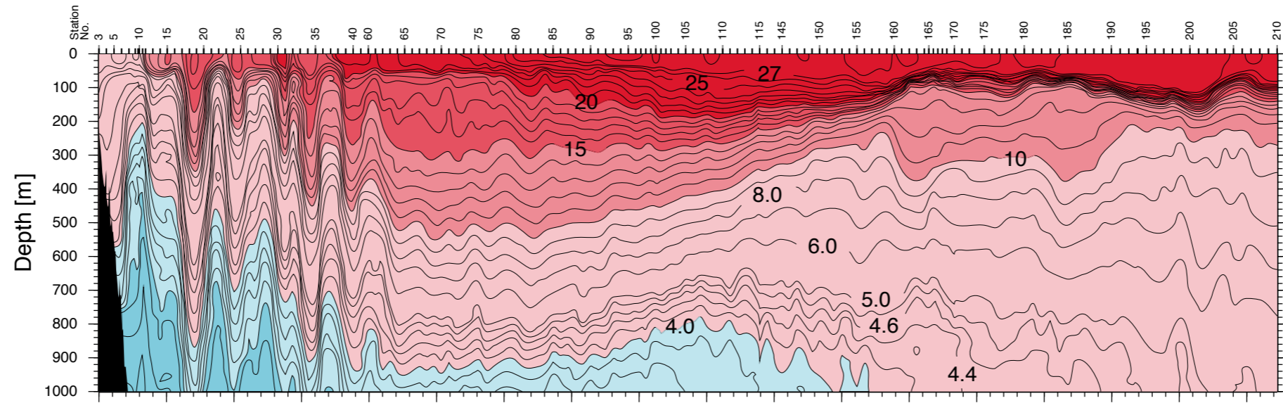
Potential Temperature [°C] for A17
